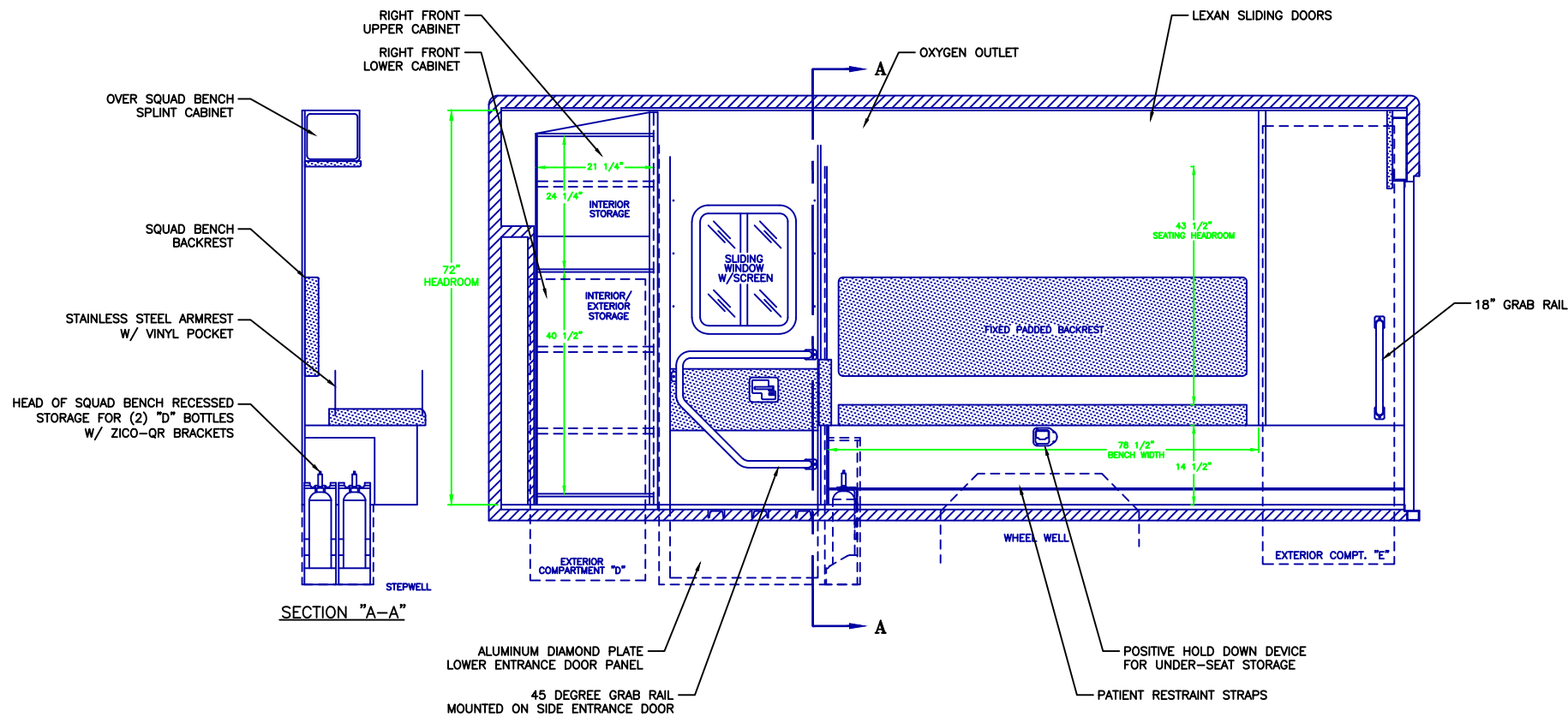
CURBSIDE VIEW
