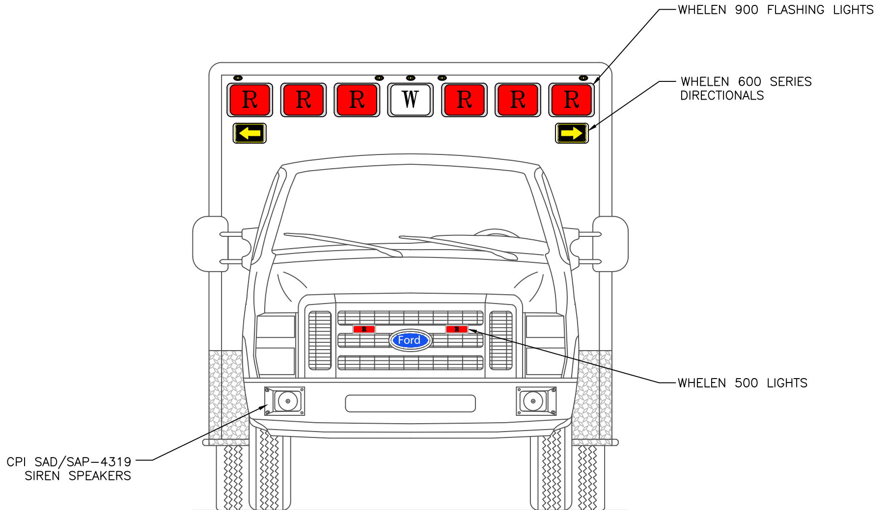
FRONT VIEW
