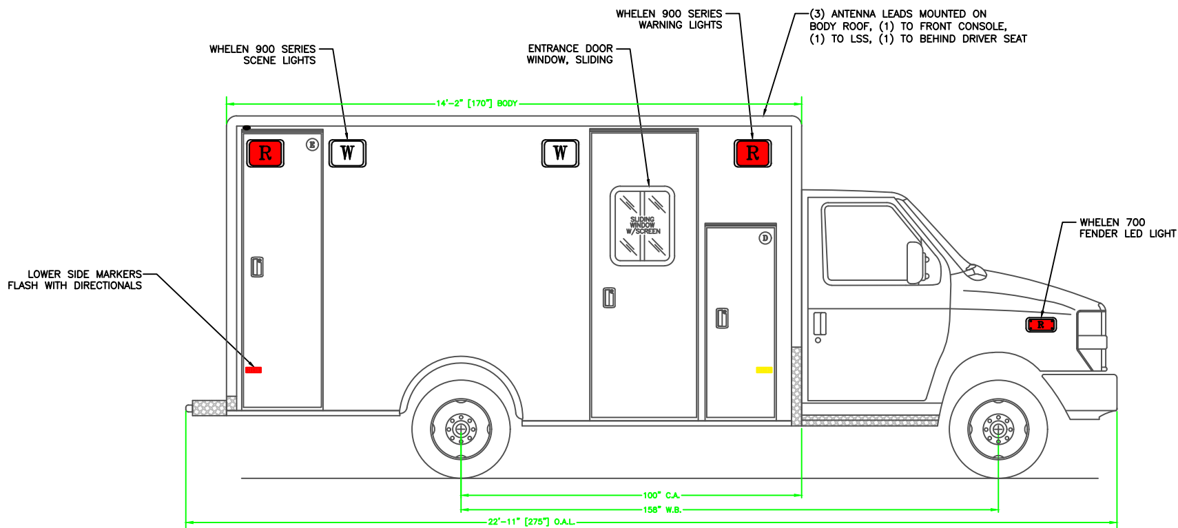
CURBSIDE VIEW
