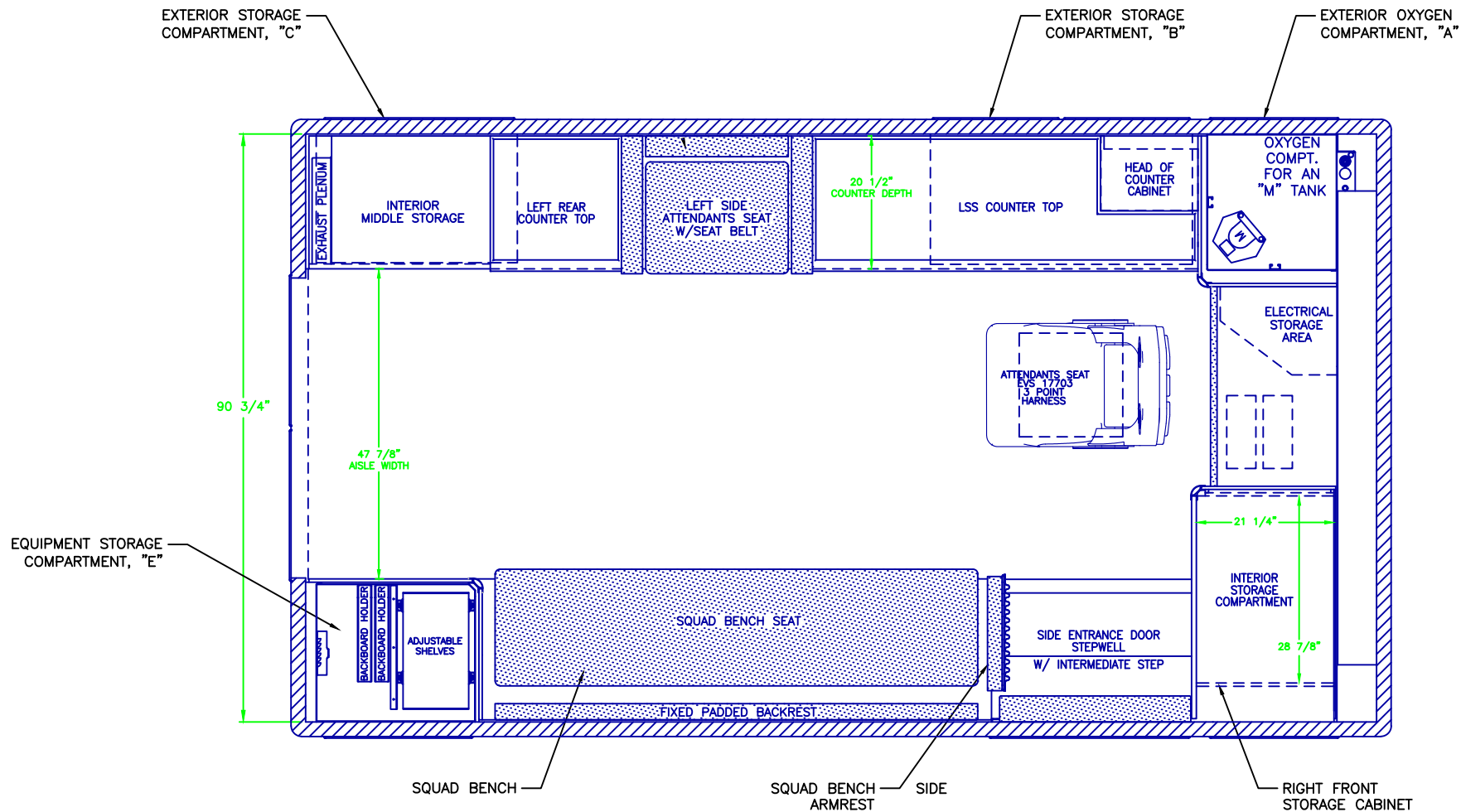
FLOOR PLAN
